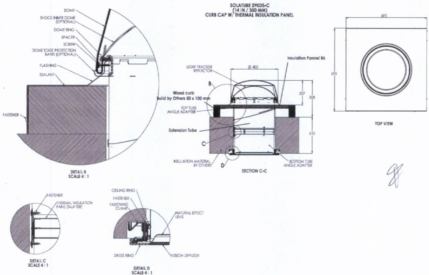
Figure 1 – Sections Solatube 290DS-C.
