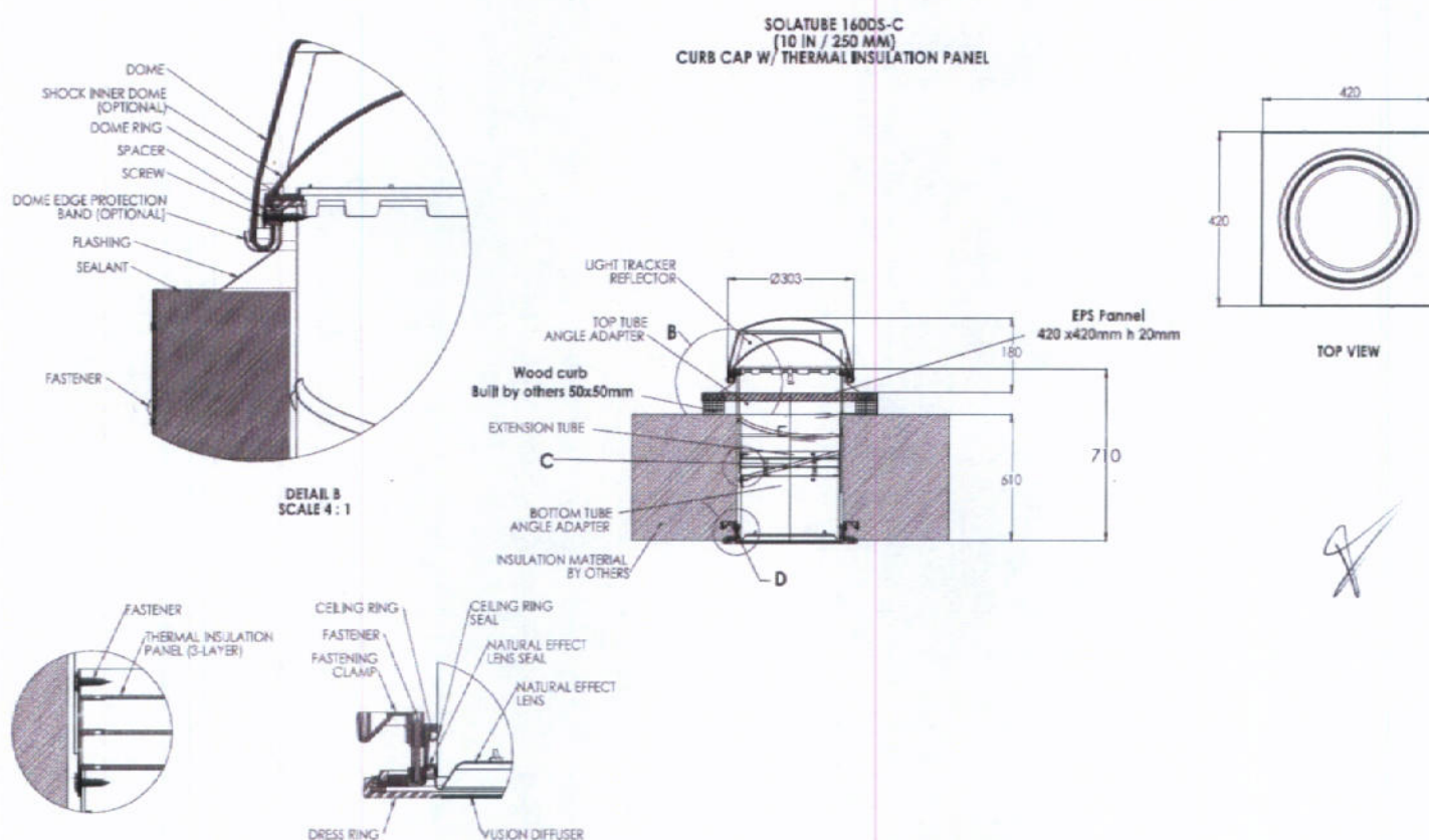
Figure 1 – Sections Solatube 160DS-C.
